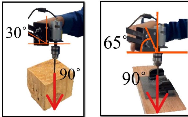
Figure 11: Different arm angle on machine
