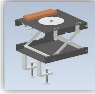
Figure 4: Scissor Jack
