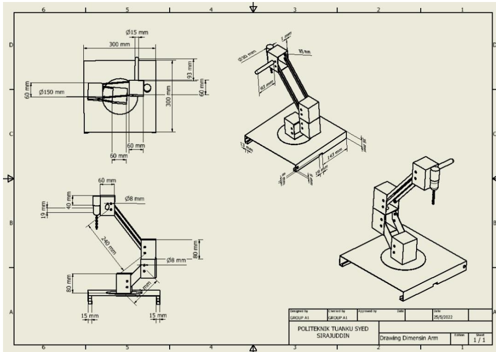
Figure 1: Project Dimensions
