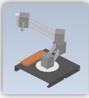
Figure 3: Arm Linkages
