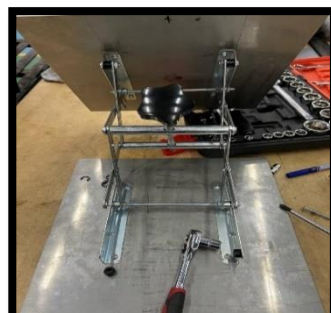
Figure 7: Scissor Jack Fabrication
