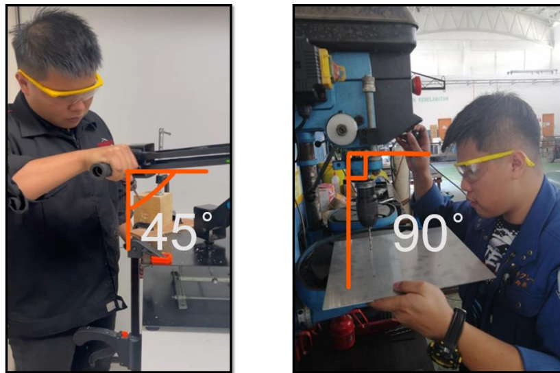
Figure 10: Different drill machine and angle
