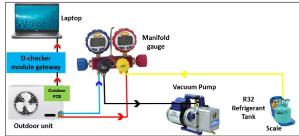
Figure 2. Refrigerant charging setup
