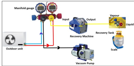
Figure 1. Recovery refrigerant setup
